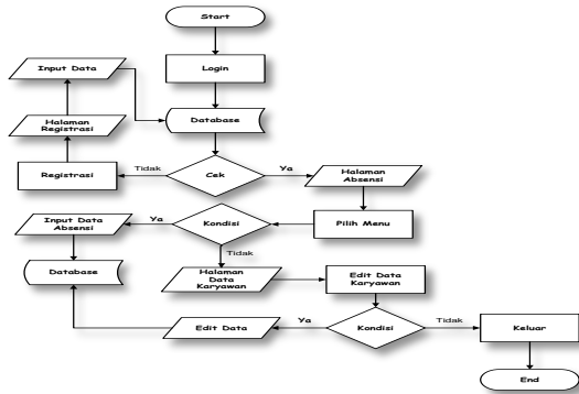
Gambar 1 Context Diagram
